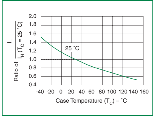
Normalized DC Holding Current versus Case Temperature
