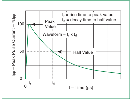
t_r \times t_d Pulse Waveform
